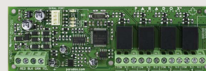
PGM4 4 PGM Expansion Module
