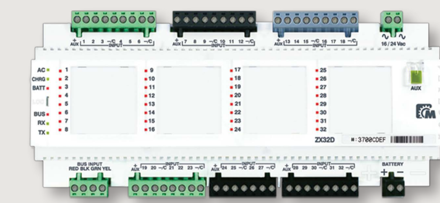
ZX32D: 32-Zone/Input Expansion Module/ 2 Amp Bus Power Supply
