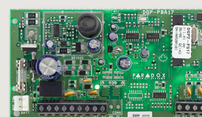
PS17 Power Supply Module
