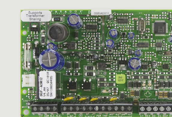
ACM12 4-Wire Access Control Module
